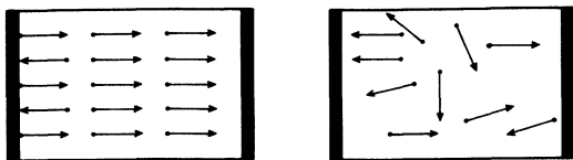
Fig. 21.3. Photons in the laser. See text
