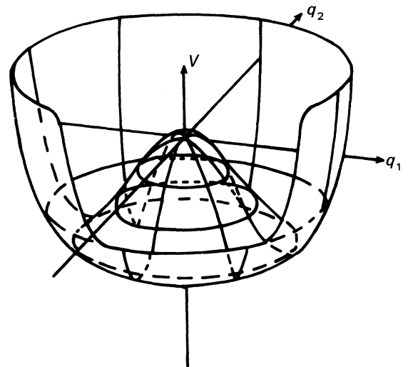
Fig. 21.10. The “effective potential” for the complex laser amplitude E = q_1 + iq_2 above the threshold
