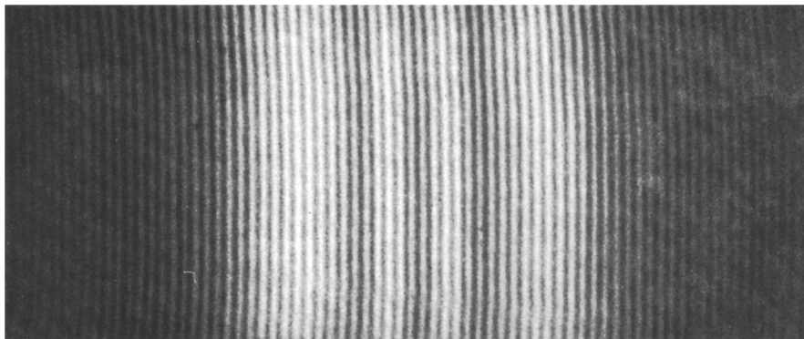
Fig. 6.10. Electron interference from the electrostatic double prism according to Möllenstedt and Düker . This image shows the measured intensity distribution on the film in Fig. 6.9; from Gerthsen, Kneser, Vogel: Physik , 13th ed. (Springer, Berlin, Heidelberg, New York 1977)
