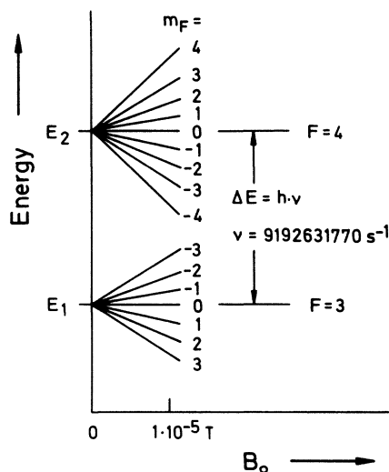
Fig. 20.24. A portion of the term scheme of the Cs atom in the ground state as a function of a weak applied magnetic field B_0 . The transition frequency used for the Cs atomic clock corresponds to the transition between the states F = 3 , m_F = 0 , and F = 4 , m_F = 0
