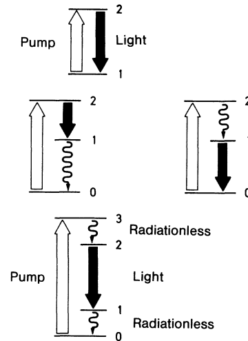
Fig. 21.4. Typical pumping schemes. Above , atom with two levels. Middle , atom with three levels: left , the upper (optical) transition is laser active; right , the lower (optical) transition is laser active. Below , atom with 4 levels. The middle (optical) transition is laser active
