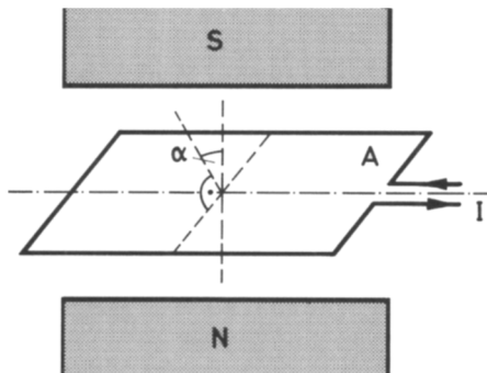
Fig. 12.3. Calculation of the potential energy of a conducting loop in a magnetic field. The magnetic moment is the product of the current I and the area vector \boldsymbol{A} . The potential energy depends on the angle \alpha between the normal to the plane of the loop and the direction of the magnetic field
