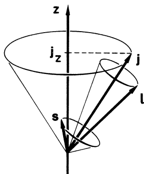
Fig. 12.12. Coupling of the vectors of spin s and orbital momentum l to give the total (resultant) angular momentum j in the vector model. The vectors s and l precess about the resultant j . In a magnetic field applied in the z direction, j precesses about z . The opening angle of the cone of precession is determined by the magnetic quantum number m_j . The figure shows the case s = 1/2 , l = 2 , j = 5/2
