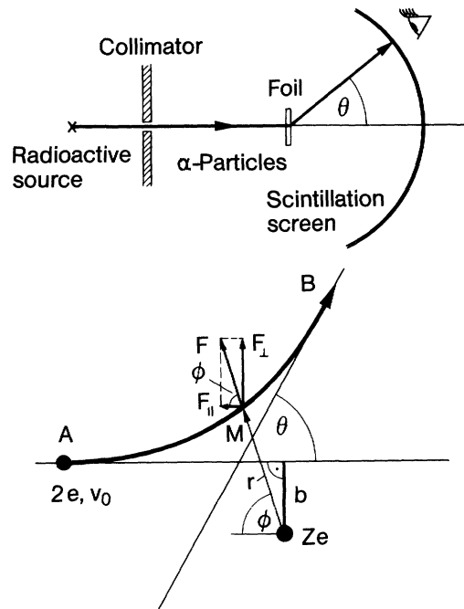
Fig. 4.7. Rutherford scattering. Upper part: Schematic illustration of the experimental setup. Lower part: The geometry of the model calculation. The alpha particle is deflected from A to B through scattering by the nucleus Ze
