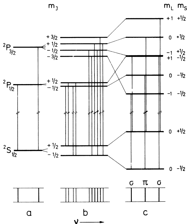
Fig. 13.15 a – c. Paschen-Back effect (c) and Zeeman effect (b) with the D_1 and D_2 lines of the neutral sodium atom (a). In the limiting case of strong magnetic fields, one observes one unshifted and two symmetrically split lines, as in the ordinary Zeeman effect
