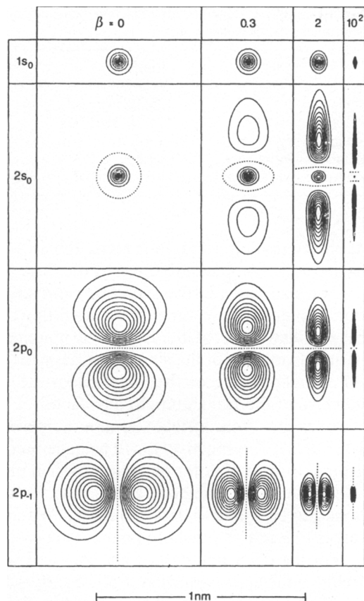
Fig. 14.12. “Contour lines” of the probability distribution of the electron of a Hydrogen atom in the xz -plane (with a decrease from maximum to zero in steps of 0.1 of the maximum) at four different values of magnetic field strength. Nodal surfaces are indicated by dashed lines. At increasing magnetic field the atomic states are compressed in the direction transverse to the field. In strongly bounded states ( 1s_0 , 2p_{-1} ) the extension parallel to the field decreases, too, while the Hydrogen-like states become heavily stretched, particularly at higher quantum numbers due to the essential orthogonality of the longitudinal wave functions in the borderline case of strong fields. (After Ruder et al., 1994)
