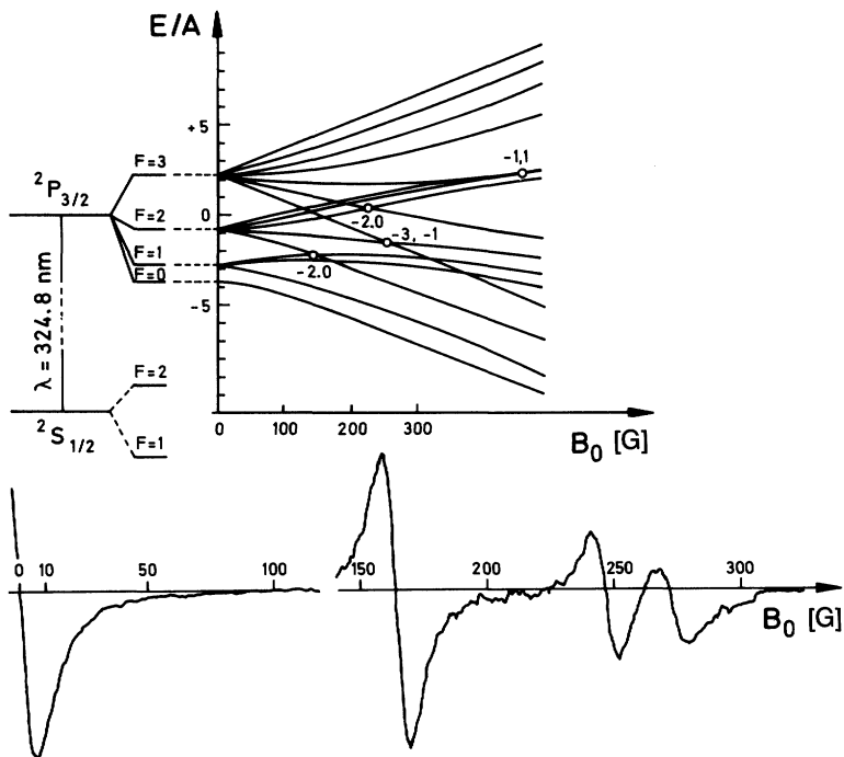
Fig. 22.10. Level-crossing spectroscopy and Hanle effect on the transition ^2S_{1/2} - ^2P_{3/2} in Cu, I = 3/2 (from Bucka et al.). In the upper portion of the figure, the energy level diagram is shown; the splitting of the excited state ^2P_{3/2} is given in units of the hyperfine structure constant A . The crossing points which are accessible to level-crossing spectroscopy are denoted by their m_F -values. The strength of the applied field B_0 is plotted along the abscissa. In the lower portion of the figure, experimental curves for the Hanle effect ( left ) and for the level crossings ( right ) are shown. For experimental reasons, the derivative of the intensity w.r.t. magnetic field dI/dB_0 is plotted rather than the intensity itself. The plots therefore are dispersion curves and the level-crossing fields B_c correspond to the zero-crossings of the curve, i.e. the points where it crosses the abscissa. At the left, one can see the Hanle effect at B_0 = 0 ; on the right, the 3 level crossings, corresponding to the crossing points (-2, 0) , (-2, 0) and (-3, -1) in the term diagram. To convert the linewidth in Gauss to the value in MHz, (13.7) is to be used
