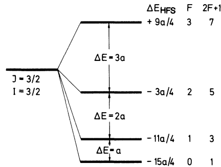
Fig. 20.5. Hyperfine splitting and the interval rule: hyperfine splitting of a state with J = 3/2 and I = 3/2 . The numerical values of the quantum number F and the degree of degeneracy 2F+1 (with respect to m_F ) are given on the right
