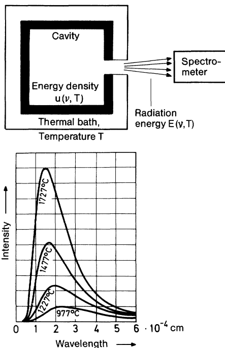
Fig. 5.3. Thermal radiation. Upper part: Schematic illustration of a cavity radiator. Lower part: Typical measured curves of the intensity distribution in the black body radiation at various temperatures
