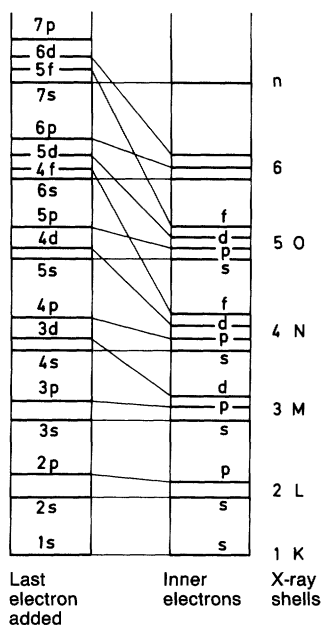
Fig. 19.3. The shell structure of the atomic energy levels and their ordering, for the last added electron and for the inner electrons. Especially stable configurations are those in which a large energy gap to the next level occurs
