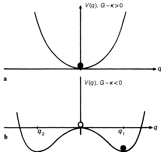
Fig. 21.9 a, b. The “effective potential” for the laser amplitude q \equiv E . a) Potential for pumping power below the threshold. b) The same above the threshold
