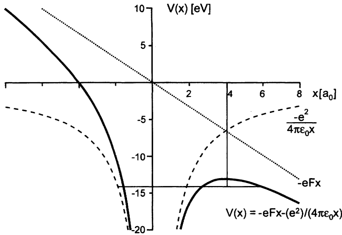
Fig. 15.11. Potential of a hydrogen atom in a static external electrical field of F = 3 \cdot 10^{10} V/m. The bound state at an energy of -13.6 eV is able to tunnel through the right potential barrier (tunnel ionization). At a slightly stronger electrical field the potential barrier on the right side will be lowered beneath the threshold value of the binding energy so the electron is no longer bonded ("over the barrier"-ionization). X-axis units are Bohr radii
