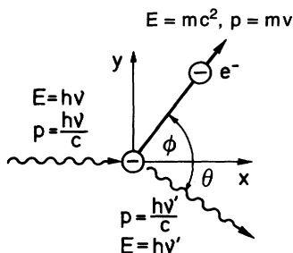
Fig. 5.9. Explanation of the Compton effect: the incident x-ray quantum with energy E = h\nu and momentum p = h\nu/c collides with an electron. In the collision, it transfers energy and momentum to the electron; the scattered x-ray quantum thus has a reduced energy h\nu' and a reduced momentum h\nu'/c
