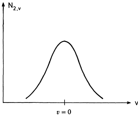
Fig. 22.4. The number of excited atoms N_2 with velocity v is represented as a function of v by a Gaussian curve, according to the Maxwell distribution
