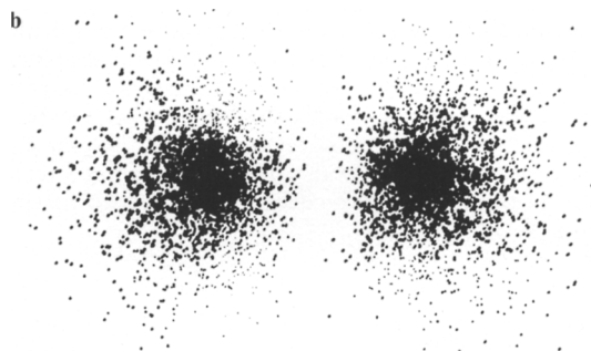
Fig. 24.7. a) The antisymmetric wavefunction \psi_- is formed by taking the difference of \phi_a and \phi_b . The occupation probability is clearly zero in the plane of symmetry between the two nuclei. b) Illustration of the density distribution of the electron in the hydrogen-molecule ion in the case of the antisymmetric wavefunction \psi_-
