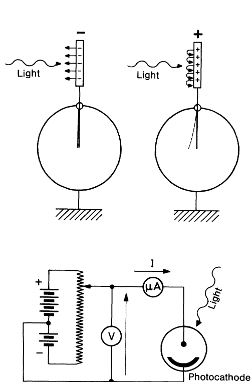
Fig. 5.6. Photoeffect. Upper part: A negatively charged electrometer is discharged upon illumination of the electrode, a positively charged one is not. Lower part: Arrangement for quantitative study of the photoeffect (voltage V , current I )
