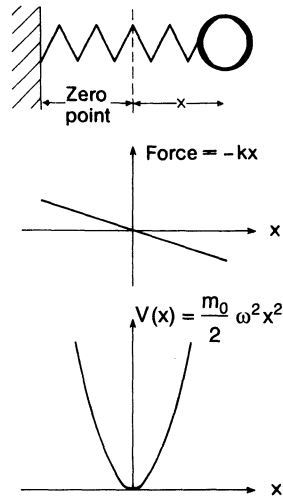
Fig. 9.5. The harmonic oscillator. Above , as an example, a point mass on a spring. Middle , force as a function of the displacement x . Below , potential energy as function of the displacement x
