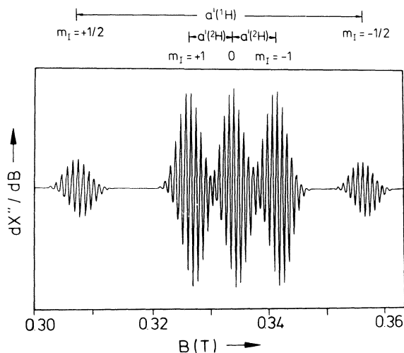
Fig. 20.15. The ESR spectrum of hydrogen atoms which are stored in interstitial sites in a KCl crystal. The two outer groups of lines belong to the transitions with \Delta m_s = 1 and m_I = +1/2 or m_I = -1/2 of the light hydrogen isotope (mass number 1, ^1\text{H} ), having a splitting a(^1\text{H}) of 500 Gauss; cf. Fig. 20.14. Each of these transitions is split into 13 equidistant lines, due to what is termed the superhyperfine structure, i.e. the interaction with the nuclear moments of the four nearest-neighbor \text{Cl}^- anions ( I = 3/2 ). The three inner groups of lines belong to the transitions with \Delta m_s = 1 and m_I = 1, 0 , or -1 of heavy hydrogen ( ^2\text{H} , deuterium, with I = 1 and g_I = 0.857 ). The splitting constant a(^2\text{H}) is smaller by the ratio of the g_I factors than that of ^1\text{H} (see J. M. Spaeth: Phys. stat. sol. 34 , 71 (1969)). In the limiting case of a strong external field B_0 , the hyperfine coupling constant a' measured by this method is identical to the isotropic hyperfine constant a as in (20.11)
