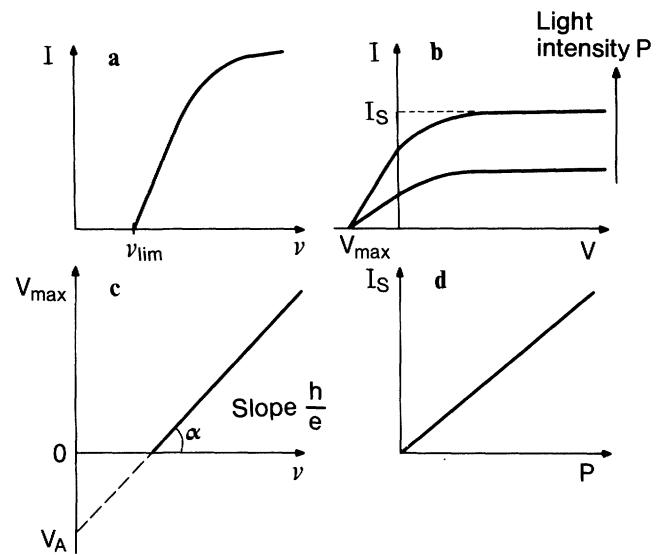
Fig. 5.7 a – d. Quantitative results for the photoeffect. a) Photocurrent I as a function of the frequency \nu of the light. Below the limiting frequency \nu_{\text{lim}} there is no longer a photocurrent. b) Photocurrent I as a function of the applied voltage V . Positive values of the voltage here mean that the irradiated electrode is the cathode . The largest negative voltage which can still be overcome by the photoelectrons (when the irradiated electrode is the anode ) is V_{\max} . The saturation current I_S is a function of the light intensity P . c) Maximum braking voltage V_{\max} as a function of the light frequency \nu ; measurement of the ratio h/e and of the work function V_A as the slope and intercept of the straight line according to (5.28). It should be remembered that in the counter-field method, both work functions, that of the cathode and that of the anode, are to be taken into account. d) Saturation current I_S as a function of the light intensity P . The current increases with the intensity
