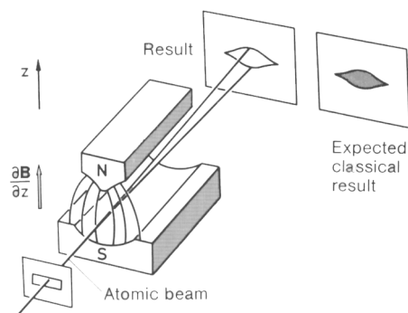
Fig. 12.10. Stern-Gerlach experiment. The atomic beam passes through an inhomogeneous magnetic field. One observes the splitting of the beam into two components. Classically, one would expect a continuous distribution
