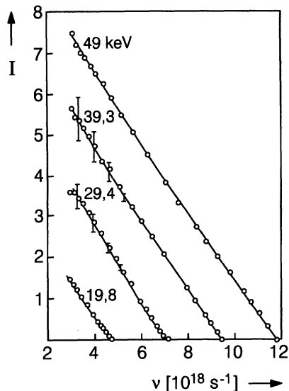
◀ Fig. 18.4. The intensity I in the x-ray bremsstrahlung spectrum as a function of the frequency for different primary energies of the electrons used for excitation. The measurement was carried out with a thick anticathode (after Kulenkampf)
