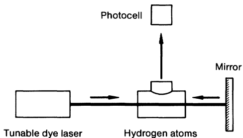
Fig. 22.9. Diagram of an experimental arrangement for two-photon spectroscopy. Two laser beams moving in opposite directions along the optical axis are passed through the gas being studied. By absorption of two photons (one from each of the oppositely propagating laser beams), an atom is raised to an excited state. Its recombination radiation is detected by the photocell, giving a measure of the strength of the absorption process
