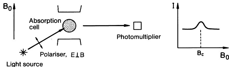
Fig. 22.11. Level-crossing spectroscopy and Hanle effect. Left, a schematic of the experimental setup. The atoms in the gas cell are excited by polarised light from a conventional light source and the resonance light (with or without polarisation analyser) is observed as a function of the magnetic field B_0 . At level-crossing fields B_c , the intensity and the polarisation of the resonance light detected by the photomultiplier change, in general. This is indicated on the right
