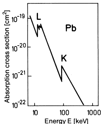
Fig. 18.12. Absorption cross section of lead for x-rays in the region of the L and K edges. The absorption coefficient is expressed in terms of the absorption cross section of an atom
