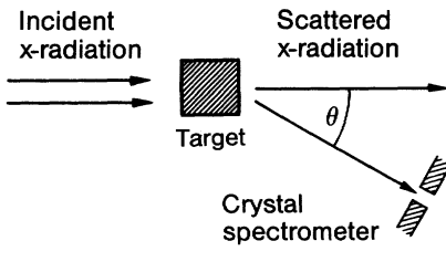
Fig. 5.8. Compton Effect. Upper part: Experimental setup. The x-radiation which is scattered by the target (e.g., a graphite block) is measured as a function of the scattering angle \theta , which is defined to be 0^\circ for undeflected radiation and 180^\circ for radiation reflected back towards the source. Lower part: Measured scattered radiation as a function of wavelength for various scattering angles. The unshifted Rayleigh-scattered radiation as well as the shifted Compton-scattered radiation are seen
