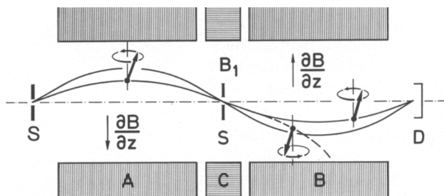
Fig. 20.16. Atomic beam resonance according to Rabi . The magnetic fields A and B are inhomogeneous, while magnet C has a homogeneous field B_0 . A high-frequency field B_1 is applied perpendicular to B_0 (S, source; D, detector)
