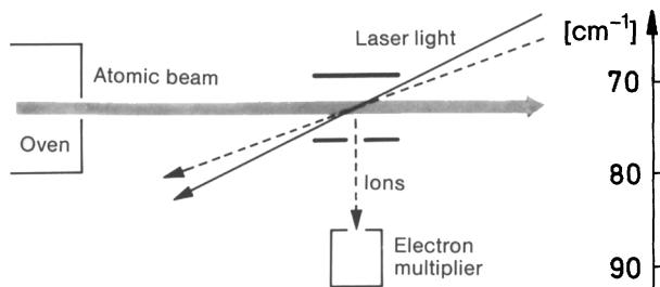
Fig. 8.16. Apparatus for the detection of Rydberg atoms. An atomic beam is crossed by several (here 2) laser beams. They cause the excitation of the atoms into Rydberg states when the sum of the quantum energies of the laser beams corresponds to the excitation energy of a Rydberg state. The Rydberg atoms are ionised in the electric field of a condenser, and the ions are then detected
