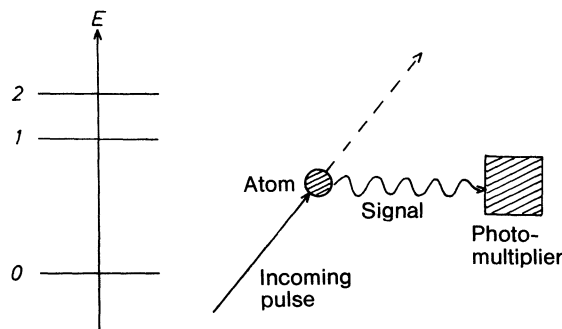
Fig. 22.2. Quantum beats. Left: Schematic energy level diagram. Right: Experimental set-up. The atom is excited by an incoming light pulse. The emitted radiation is measured in another direction with a photomultiplier. Typical experimental results are shown in Fig. 22.3
