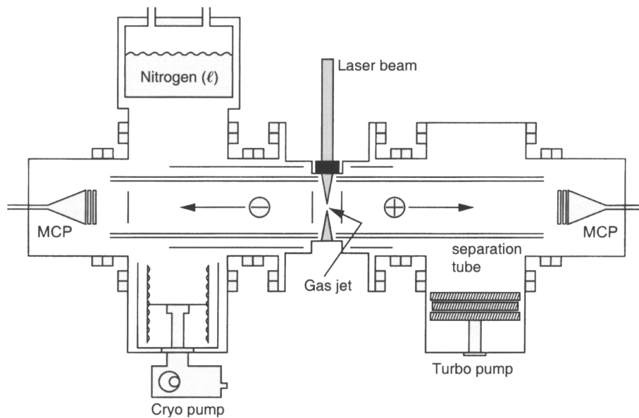
Fig. 15.12. Time-of-flight mass spectrometer: the apparatus will be evacuated by a turbo pump and a cryo pump. In addition, the flight tunnel may be cooled with liquid nitrogen. In the field-free flight path electrons drift towards the left microchannel plate detector while ions will be accelerated towards the right microchannel plate detector via a suction voltage. By means of delayed suction ions and electrons may be measured simultaneously
