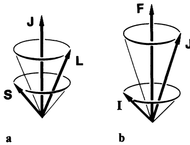
Fig. 20.3. a) Coupling of the S (spin) and L (orbital angular momentum) vectors to a total electron angular momentum vector J for the electron shell. b) Coupling of the J (electron angular momentum) and I (nuclear angular momentum) vectors to the total angular momentum F of the atom
