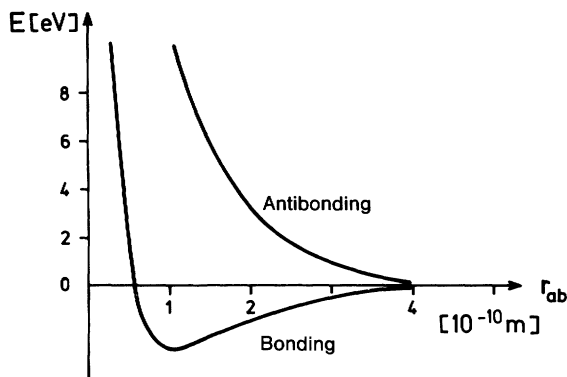
Fig. 24.8. The energy E of the hydrogen-molecule ion, taking the Coulombic repulsion between the two nuclei into consideration. The energy curves are plotted to show their dependence on the internuclear distance r_{ab} for the bonding and the antibonding states
