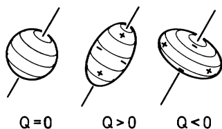
Fig. 20.25. Charge distributions in nuclei. If the nucleus is spherically symmetric, Q = 0 . In the case of a cigar-shaped (prolate) nuclear charge distribution, Q is positive; for a pincushion shape (oblate), Q is negative. As a rule, large nuclear quadrupole moments are positive. The symmetry axis of the distribution is the direction of the nuclear spin vector I
