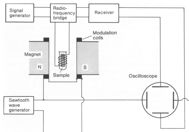
Fig. 20.18. Diagram of a simple nuclear spin resonance apparatus. The sample is placed in a glass tube between the poles of a homogeneous magnet. The high-frequency B_1 field is applied across a bridge and an induction coil. For better detection of resonance, the B_0 field can also be modulated by an additional coil
