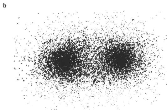
Fig. 24.6. a) The symmetric wavefunction \psi_+ is formed by superposing the wavefunctions \phi_a and \phi_b . Because of the overlap between \phi_a and \phi_b , the occupation probability for \psi_+ between the two nuclei is increased. b) Illustration of the density distribution of the electron in the \psi_+ state
