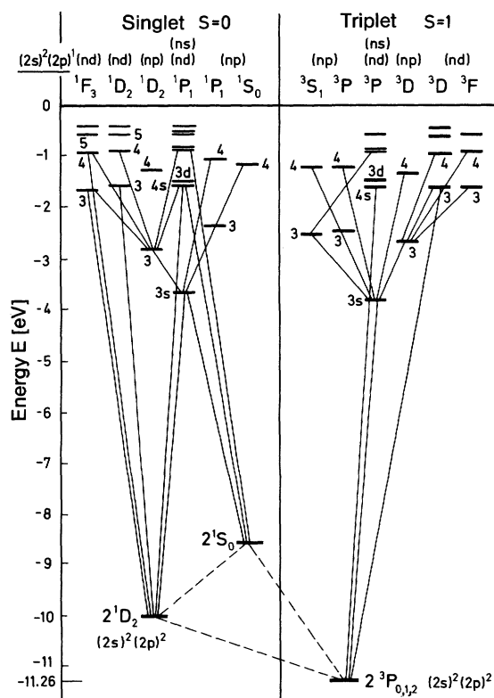
Fig. 17.5. Term diagram for the carbon atom (only simple terms, no J splitting). Carbon has a singlet and a triplet system. The configuration of the valence electrons is given at the top
