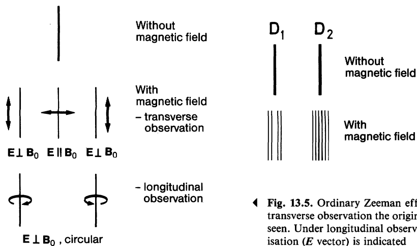
Fig. 13.6. Anomalous Zeeman effect, here using the sodium D lines. The D_1 line splits into four components, the D_2 line into six in a magnetic field. The wavelengths of the D_1 and D_2 lines are 5896 and 5889 \text{\AA} ; the quantum energy increases to the right in the diagram
