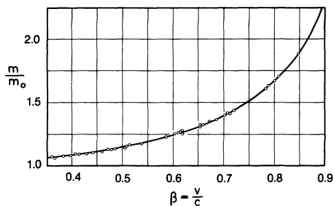
Fig. 6.5. Experimental values for the mass of the electron as a function of its velocity (test of the Lorentz formula). The mass m , in units of the rest mass m_0 , is plotted against the velocity in units of the velocity of light, v/c
