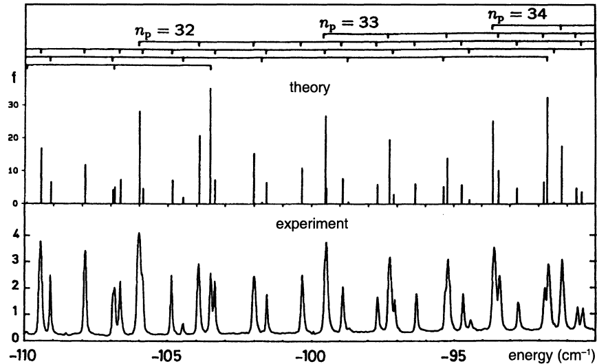
Fig. 14.5. Deuterium Rydberg atoms in a magnetic field of strength 6.0 T. The figure shows a section from a comparison of the spectrum of theoretical oscillator strengths and the experimental photo absorption spectrum for \Delta m = 0 of the Balmer transitions after m = 0 at Rydberg states of even parity. Oscillator strengths are given in units of 10^{-6} , experimental intensities are given in arbitrary units. (After Holle et al., 1987)
