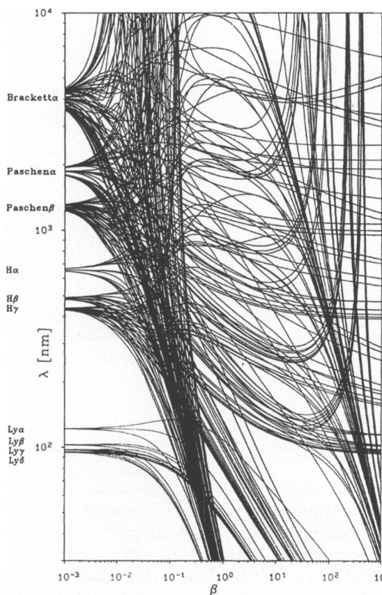
Fig. 14.11. Wavelength spectrum of hydrogen atoms from soft X-rays (30 nm) to the far infrared (10 000 nm) as a function of the magnetic field in the interval 470 T through 4.7 \times 10^8 T, plotted in doubly logarithmic scale. All possible transitions between states of (field-free) principle quantum numbers n < 5 and n' \neq n have been included. Effects due to the finite nature of the proton mass have been taken into account. The two line bundles that exhibit a sharp downward bend correspond to cyclotron-like transitions of electrons (bundle to the left) and protons (bundle to the right). The stationary lines in the intermediate region are recognizable particularly well if viewed at an angle. (After Ruder et al., 1994)
