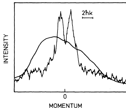
Fig. 22.14. The momentum distribution of atoms in the direction of the laser beam, for helium-4 atoms which have been cooled by the velocity-selective coherent population trapping method. The width of each peak is smaller than the momentum \hbar k of a single photon, which is an indication of cooling to below the recoil limit. The momentum distribution of uncooled atoms is shown by the bold-face curve. (Redrawn from A. Aspect, E. Arimondo, R. Kaiser, N. Vansteenkiste, and C. Cohen-Tannoudji: Phys. Rev. Lett. 61 , 826 (1988))
