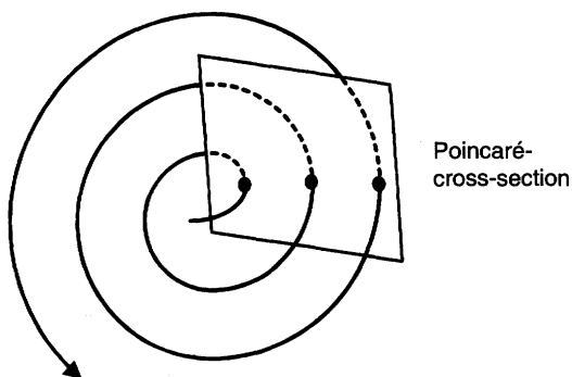
Fig. 14.7. Visualization of a Poincaré cross-section that penetrates the trajectory several times (in the limit of long periods of time an infinite number of times)
