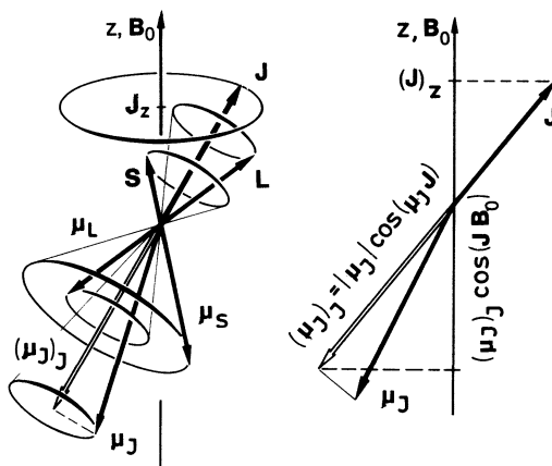
Fig. 13.11. Left: The relation between the angular momentum J , the magnetic moment \mu_J and their orientation with respect to the magnetic field B_0 for strong spin-orbit coupling, cf. also Fig. 13.13. The angular momentum vectors S and L combine to form J . Likewise, the associated magnetic moments \mu_L and \mu_S combine to \mu_J . Because spin and orbital magnetism have different gyromagnetic ratios, the directions of the vectors J and \mu_J do not coincide. What can be observed is the projection of \mu_J on J , as the time average of many precession cycles. That is, one observes the component (\mu_J)_J , which is therefore represented as \bar{\mu}_J or \bar{\mu}_S , see the right-hand diagram. In the one-electron system, lower case letters can be used instead of S , L and J , as is done in the text. Right: The projection of \mu_J on the vector J is (\mu_J)_J , see Fig. 13.14. The projection of (\mu_J)_J on B_0 is calculated using the Landé factor. Because the angular momenta S and L are strongly coupled, the vector \mu_J precesses rapidly around the negative extension of the vector J . Only the time average (\mu_J)_J in the J direction can be observed. This precesses slowly, because of weak coupling, around the axis of B_0 . The magnetic energy is the product of the field strength B_0 and the component of (\mu_J)_J in the direction of B_0 , i.e. (\mu_J)_{J,z} or (\bar{\mu}_J)_z \cdot B_0 . Lower case letters can be used instead of S , L , J in the one electron system.
