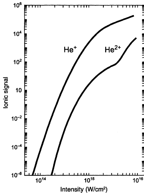
Fig. 15.13. A laser ionizes neutral helium (cf. Fig. 15.12.). The \text{He}^+ ions generated by the process and the \text{He}^{2+} ions generated at higher intensities get measured as a function of the laser intensity. (After B. Walker et al., Phys. Rev. Lett. 73, 1227 (1994))
