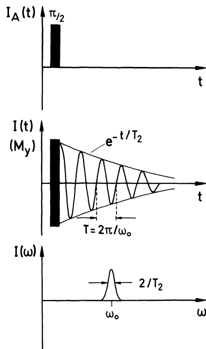
Fig. 20.19. Pulsed nuclear magnetic resonance. ( Upper part ) High-frequency pulses of frequency \omega_0 are used to excite the resonance, e.g. 90^\circ pulses. The measurement is repeated many times and summed (signal averaging). ( Middle part ) The time evolution I(t) of the y component of the nuclear magnetisation, M_y , is observed. The envelope decays with the time constant T_2 when, as here assumed, only one species of equivalent nuclear spins (e.g. protons) are present in the sample. This time constant, which we have denoted by T_2 for simplicity, is more precisely called T_2^* , since it may contain T_1 in addition to the transverse relaxation time T_2 defined in Sect. 14.5. ( Lower part ) Through Fourier transformation of the observed time spectrum I(t) , one obtains the nuclear magnetic resonance spectrum I(\omega) , which is a single line in the case of one equivalent species of nuclear spins
