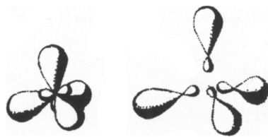
Fig. 24.12. Left: The density distributions of the four electrons in the case of tetragonal ( sp^3 -) hybridisation of carbon. Right: Exploded view
