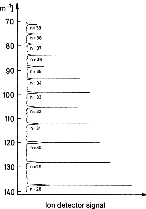
Fig. 8.17. An example of the detection of Rydberg states of the lithium atom with n = 28 to 39, measured with an apparatus like that shown in Fig. 8.16. The distance (in wave number units) to the series limit is plotted as the ordinate
