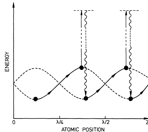
Fig. 22.13. An atom moving within the laser configuration of Fig. 22.12 climbs out of a potential valley onto a maximum before it is optically pumped to the minimum of another valley. On the average, the atom experiences more climbs than drops, and the resulting net energy loss cools it. The effect is near its optimum conditions in the case shown here, since the atom moves one-fourth of a wavelength in the mean time \tau_p ; this is the average time which the atom must wait before it experiences another optical pumping cycle. (After Claude N. Cohen-Tannoudji and William D. Phillips: Physics Today , pp. 33–40 (1990))
