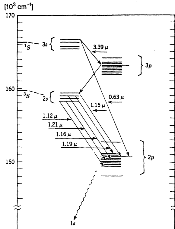
Fig. 21.6. Splitting and transition scheme for the energy levels of helium (left ordinate) and neon (centre). The ground state of neon, which is not shown here, has the electron configuration 1s^2 2s^2 2p^6 . In the states shown, one of the six 2p electrons is excited. If we give only the configuration of the six outermost electrons, then the abbreviations 1s , 2s , and 3s stand for 2p^5 3s , 2p^5 4s and 2p^5 5s , respectively. Each of these states consists of 4 terms. The abbreviations 2p and 3p stand for 2p^5 3p and 2p^5 4p , each of which has 10 terms
