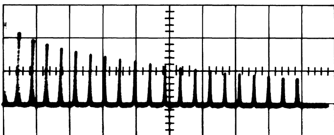
Fig. 15.9. A series of spin echos obtained from protons in ordinary water. In this method, a 90^\circ pulse is applied at time t = 0 , and is followed at times \tau, 3\tau, 5\tau, \dots, (2n-1)\tau by a 180^\circ pulse. The echoes are observed at the times 2\tau, 4\tau, \dots, 2n\tau ( n an integer). It can be shown that the height of the peaks decays according to the formula f(n) = \exp(-2n\tau/T_2) . From A. Abragam: The Principles of Nuclear Magnetism (Oxford, 1962)
