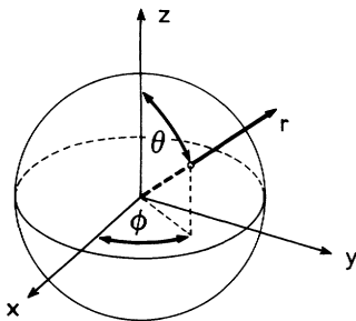
Fig. 10.1. Illustration of spherical polar coordinates
