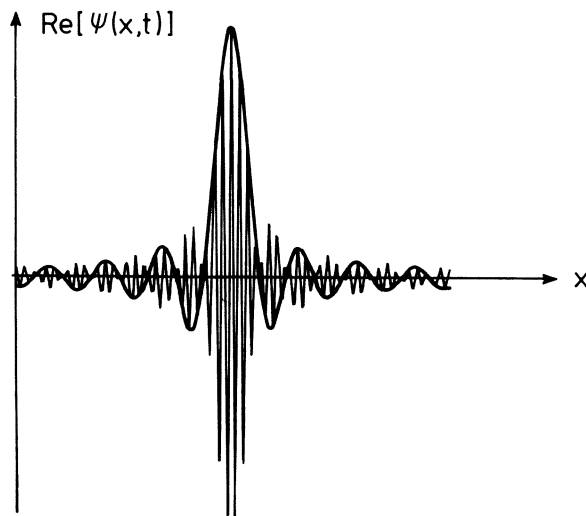
Fig. 7.3. The real part of \psi(x, t) as a function of the position x . The rapid oscillations are described by \cos(k_0 x - \omega_0 t) with t fixed. The envelope is given by \sin[(\omega' t - x)\Delta k]/(\omega' t - x) with t fixed. Note that the scale of the x axis has been greatly reduced in comparison to Fig. 7.2
