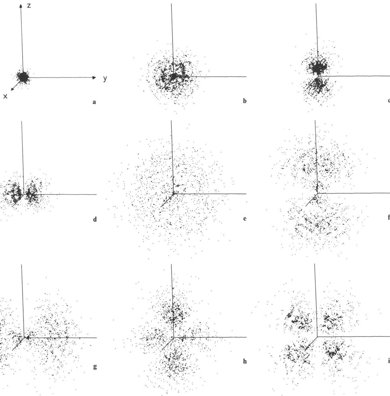
Fig. 10.4 a–i. The density distribution (= localisation probability density |\psi|^2 ) of the electron in the H atom represented by the density of dots (according to H. Ohno ). The wavefunctions represented are:
