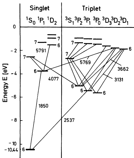
◀ Fig. 17.7. Simplified energy diagram of the mercury atom as an example of a heavy atom with term symbols corresponding to LS -coupling. The wavelengths [ \text{\AA} ] of a few of the more important lines are given. The strongest line in the spectrum of a mercury lamp is the line at 2537 \text{ \AA} which results from the intercombination of the 6^1S_0 and the 6^3P_1 states. Intercombination between terms of different multiplicity is strictly forbidden in light atoms. In heavy atoms it is possible. This line corresponds to the energy loss of 4.9 \text{ eV} in the Franck-Hertz experiment, Sect. 8.8
