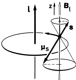
Fig. 12.15. Precession of the spin about the magnetic field \mathbf{B}_l associated with the orbital angular momentum, with the components s_z and \mu_{s,z}
