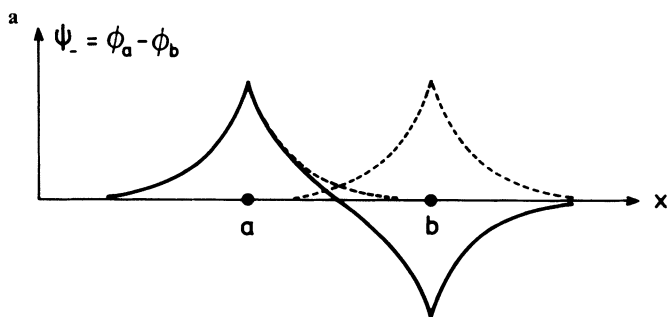
Fig. 24.7. a) The antisymmetric wavefunction \psi_- is formed by taking the difference of \phi_a and \phi_b . The occupation probability is clearly zero in the plane of symmetry between the two nuclei. b) Illustration of the density distribution of the electron in the hydrogen-molecule ion in the case of the antisymmetric wavefunction \psi_-
