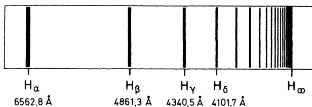
Fig. 8.3. Balmer series in the hydrogen emission spectrum. The convergence of the lines to the series limit H_\infty is clearly seen
