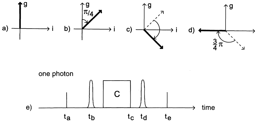
Fig. 22.17a–e. Similar to Fig. 22.16, but with one photon present. (a) In the initial state, the atom is in level g . (b) The first pulse rotates the vector (c_g, c_i) by \pi/4 . (c) The interaction with the photon reflects the vector in the i -axis. (d) The second pulse rotates the vector by 3\pi/4 , so that (apart from a sign) the state i is again reached. Finally, the atomic state – here i – is measured. (e) Temporal sequence of pulses
