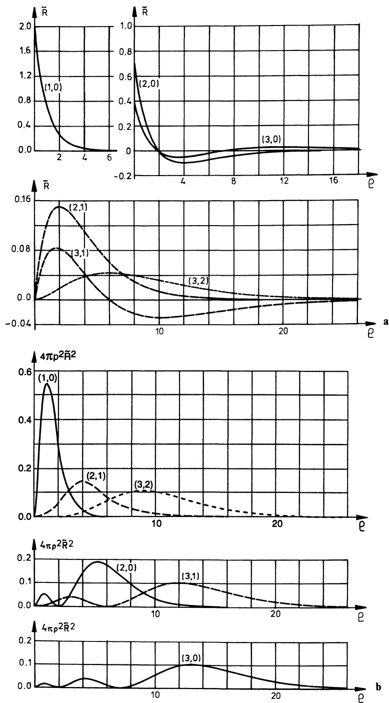
Fig. 10.3. a) The radial wavefunctions \tilde{R}(\rho) = R(r) of the hydrogen atom (10.77) are plotted vs the dimensionless coordinate \rho . The indices on the curves, (1,0), (2,0) etc. correspond to (n, l) where n is the principal quantum number and l the angular momentum quantum number. b) The corresponding probability densities in the radial coordinate, i.e. 4\pi\rho^2\tilde{R}^2(\rho) are plotted against the dimensionless coordinate \rho
