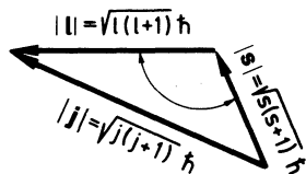
Fig. 12.16. Vector addition of the angular momentum vectors to the total angular momentum j , explanation of (12.29)
