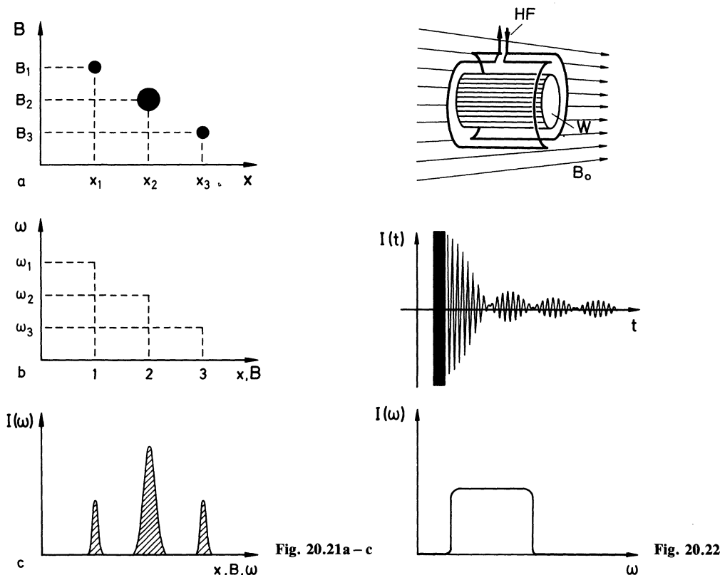
Fig. 20.21 a – c. Nuclear resonance of three samples with the same nuclei, e.g. protons, in a field gradient; illustrating position-resolved nuclear magnetic resonance. (a) In a field gradient dB/dx , each position x_1, x_2 , and x_3 corresponds to a different field strength B_1, B_2 , and B_3 . Samples 1, 2, and 3 (with 2 larger than 1 and 3) are thus in regions of differing field strength. (b) Through the resonance condition \omega = \gamma B_0 , each position x_1, x_2 , or x_3 corresponds to a particular resonance frequency \omega_1, \omega_2 , or \omega_3 . (c) The intensity of the NMR signal is a measure of the number of nuclei with the given resonance frequency ( \omega_1, \omega_2, \omega_3 ). A unique correspondence between the measured spectrum and the spatial arrangement of the nuclei exists
