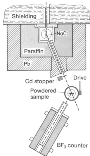
Fig. 6.12. Neutron spectrometer according to E. V. Wollan , C. G. Shull , Phys. Rev. 73 , 830 (1948). The neutrons are monochromatised by reflection from a NaCl crystal. When diffracted from a polycrystalline sample, they generate interference rings according to Debye-Scherrer . They are measured by means of a \text{BF}_3 counter. This is a historical spectrometer. Modern instruments, however, contain the same basic elements. A single crystal can also be the object of investigation.
