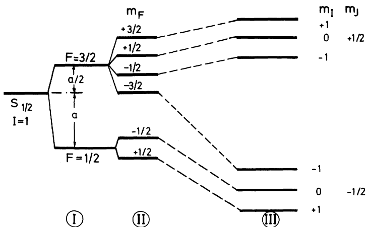
Fig. 20.11. Hyperfine structure of an S_{1/2} state with I = 1 , without applied field (I); in a weak applied field, corresponding to the Zeeman effect with hyperfine structure (II); in a strong applied field, the Paschen-Back effect with hyperfine structure (III). In making the transition from a weak to a strong applied field, the Zeeman effect of the hyperfine structure thus becomes the hyperfine structure of the Zeeman effect
