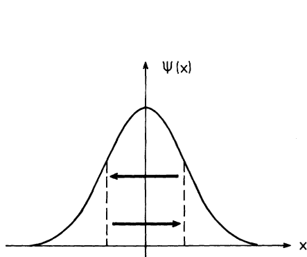
Fig. 16.1. Example of a symmetric wavefunction. When reflected through the \Psi axis, \Psi is converted into itself
