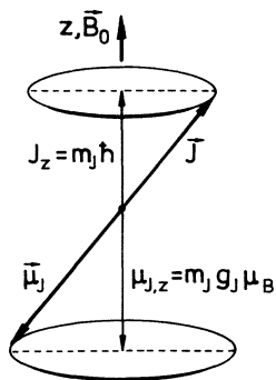
Fig. 13.9. Precession of \mathbf{J} and \boldsymbol{\mu}_j about the direction of the applied field B_0 : ordinary Zeeman effect, i.e., \mathbf{J} = \mathbf{L}
