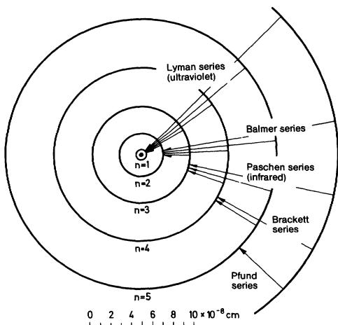
Fig. 8.5. Schematic representation of the Bohr atomic model, showing the first five spectral series
