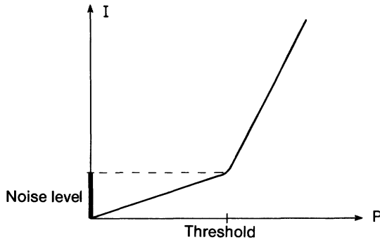
Fig. 21.8. The emission behaviour of a single-mode laser. Abscissa: pumping power input. Ordinate: emission power (in a single mode). Below the threshold, i.e. the critical pumping power, the light consists of spontaneously generated wave trains (“noise”). If this is ignored, the emitted radiation is equal to zero. Laser activity begins at the threshold
