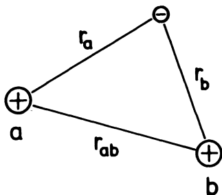
Fig. 24.1. Overview of the hydrogen-molecule ion. The two nuclei are denoted as a and b , their distance apart as r_{ab} . r_a and r_b give the distance of the electron from nucleus a and from nucleus b , respectively
