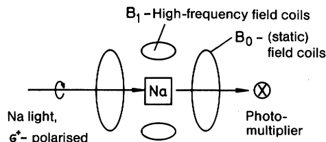
Fig. 13.18. Optical pumping of the transition ^2S_{1/2} - ^2P_{1/2} of the sodium atom. In the field B_0 , the terms split up into Zeeman terms with m_j = \pm 1/2 . Only atoms in the ground state m_j = -1/2 absorb the \sigma^+ light with which the sample is irradiated. \pi transitions occurring in emission from the excited state lead to an increase in the population of atoms in the ground state with m_j = +1/2 . With the high-frequency field, transitions from m_j = +1/2 to m_j = -1/2 are induced, increasing the number of atoms which are able to absorb the pumping light
