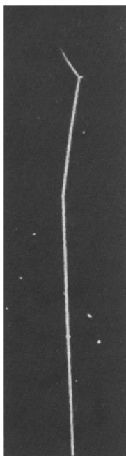
Fig. 4.3. Cloud chamber photograph of the track of an alpha particle, by Wilson . The particle passes through several cm of air without noticeable deflection. At the end of the track, we see two deflections; at the second, we can also see the short track of the target nucleus, which was accelerated to the right by the collision. [From W. Finkelburg: Einführung in die Atomphysik , 11,12th ed. (Springer, Berlin, Heidelberg, New York 1976) Fig. 3]
