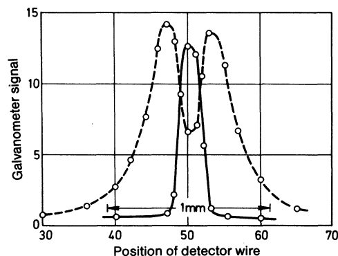
Fig. 12.11. Stern-Gerlach experiment. Observed intensity distribution of an atomic beam with and without an applied magnetic field, ^2S_{1/2} state [from H. Kopfermann: Kernmomente , 2nd ed. (Akademische Verlagsgesellschaft, Frankfurt 1956)]
