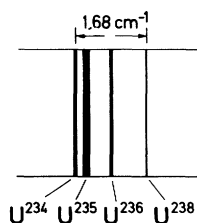
Fig. 20.1. Experimental example of the isotope effect: the isotopic splitting of the 4244.4 Å line in the uranium spectrum, observed in the 6th order in a 9m grating spectrograph. [After H. G. Kuhn: Atomic Spectra (Longmans, London 1962, Plate 18)]
