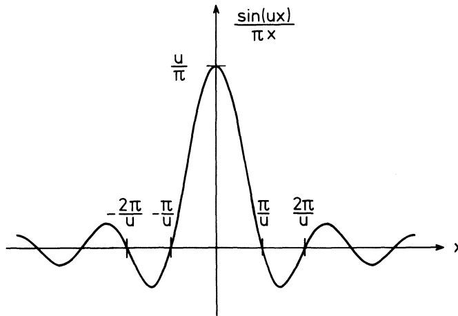
Fig. A.2. The function \sin(ux)/\pi x plotted against x . If we allow u to go to the limit infinity, the value of the function at x = 0 becomes larger and larger. At the same time, the position of the zero-crossing moves towards x = 0
