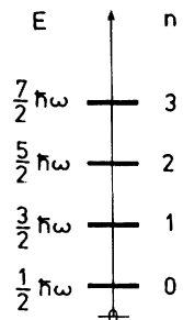
Fig. 9.7. The energy levels of the harmonic oscillator
