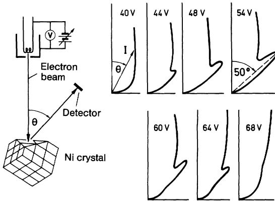
Fig. 6.7. Electron interference experiment of Davisson and Germer . Left: Diagram of the apparatus. The electrons accelerated through the voltage V are reflected from selected surfaces of a single crystal of nickel and recorded as a function of the reflection angle \theta . Right: Angular distribution of reflected electrons at various accelerating voltages. The diagrams shown are polar plots in which the distance from the zero point to the curve corresponds to the intensity of reflection at the corresponding angle. There is a maximum at a scattering or reflection angle of about 50^\circ , due to interference
