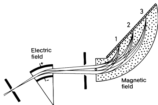
Fig. 3.4. A focussing mass spectrograph as designed by Aston . The points 1, 2, and 3 denote the points at which three types of particles with three different values of m/e are collected
