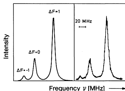
Fig. 20.9. Three components of the hyperfine-split D_2 line of sodium (Fig. 20.7), measured by recording the resonance radiation of sodium atoms in an atomic beam irradiated by light from a narrow-band, variable-frequency dye laser. The \Delta F values for the ground and excited state are given. The curve on the left is calculated from the natural linewidth, the curve on the right was observed experimentally. The measured (15 MHz) and calculated natural linewidths are very close [from Lange et al.: Opt. Commun. 8, 157 (1973)]
