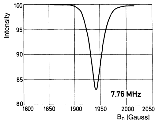
Fig. 20.17. Data curve from the Rabi atomic beam resonance experiment. The intensity at the detector is at a minimum (for a constant frequency of the field B_1 ) when the homogeneous field B_0 of magnet C fulfills the resonance condition. The curve shown here is for fluorine nuclei
