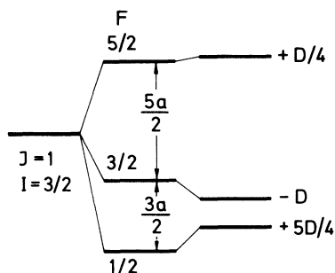
Fig. 20.26. Quadrupole shift of the hyperfine levels for a state with J = 1 and I = 3/2 . The shift indicated corresponds to a positive quadrupole moment. The constant D is equal to the factor (eQ)(\partial^2 V/\partial z^2) in (20.23). The expected splitting pattern, given by the interval rule, is modified by the quadrupole interaction
