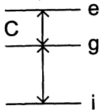
Fig. 22.15. The level scheme of an atom for nondestructive detection of a photon
