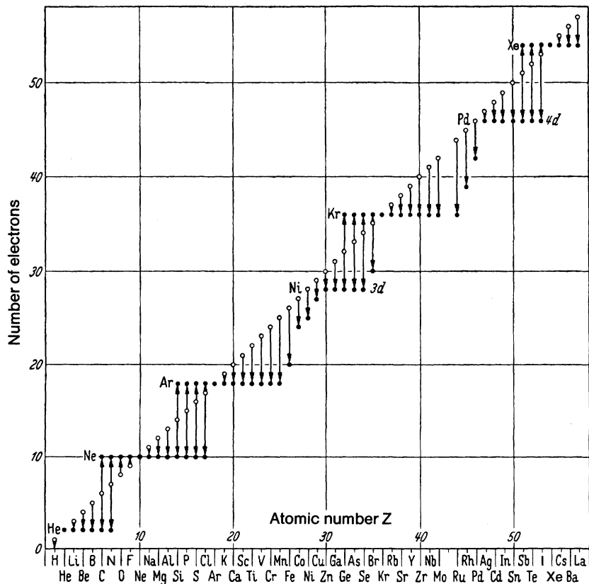
Fig. 19.1. Electronic shells of the ions of atoms, following Kossel , 1916. The number of electrons is plotted against the nuclear charge number for atoms and for the ions which are preferentially formed from those atoms in chemical bonding. The electronic shells of the atoms are depleted or filled up to the electron numbers indicated by arrows in the diagram when ions are formed. With the exceptions of nickel and palladium, the preferred electron numbers are those of the noble gases. [From K. H. Hellwege: Einführung in die Physik der Atome , Heidelberger Taschenbücher, Vol. 2, 4th ed. (Springer, Berlin, Heidelberg, New York 1974) Fig. 61]
