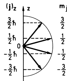
Fig. 12.13. Directional quantisation: for the z component of the angular momentum j , only certain discrete values are allowed. They are denoted by the magnetic quantum number m_j . For the case illustrated, j = 3/2 , the magnitude of the vector is |j| = \sqrt{(3/2)(5/2)} \hbar . Four orientations are allowed: m_j = 3/2, 1/2, -1/2, -3/2
