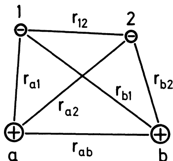
Fig. 24.9. Overview of the hydrogen molecule. The two nuclei are denoted by indices a and b , the two electrons by indices 1 and 2. The distances between the nuclei, between the electrons, and between electrons and nuclei, and the notations used for them, are shown in the sketch
