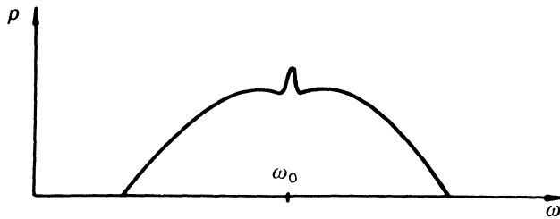
Fig. 22.6. Burning a hole in the absorption line produces a peak in the emitted radiation, which is shown here as a function of the frequency of the laser field. The width of the peak corresponds to the natural linewidth
