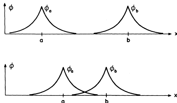
Fig. 24.3. Upper portion: The wavefunction \phi_a of an electron which is moving in the field of nucleus a and the corresponding wavefunction \phi_b for the electron in the neighbourhood of nucleus b . Lower portion: If the distance between nuclei a and b is reduced, the two wavefunctions \phi_a and \phi_b begin to overlap
