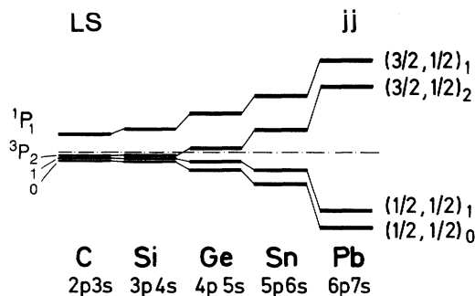
Fig. 17.9. Transition from LS coupling in light atoms to jj coupling in heavy atoms in the series C-Si-Ge-Sn-Pb. In carbon the ^3P_0 - ^3P_1 and ^3P_1 - ^3P_2 distance are 20 and 40 \text{ cm}^{-1} , while the ^1P_1 - ^3P_2 distance is 1589 \text{ cm}^{-1} . The term nomenclature is that of LS coupling for carbon, and of jj coupling for lead. The quantum symbols of the two outermost electrons are given. The symbol (3/2, 1/2)_1 means j_1 = 3/2, j_2 = 1/2, J = 1
