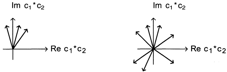
Fig. 23.2. Spreading of the phase angles. In the end, the vectors mutually cancel
