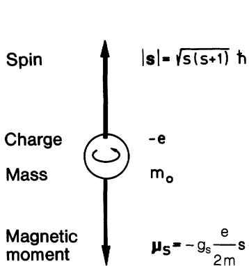
Fig. 12.7. Spin and magnetic moment of the electron
