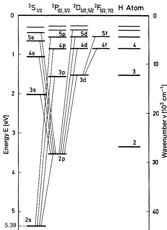
Fig. 11.5. Term diagram of the lithium atom with the most important transitions. This is called a Grotrian diagram. The term symbols given above the figure will be explained in detail in Chaps. 12 and 17. At the right, for comparison, the term scheme of hydrogen is shown
