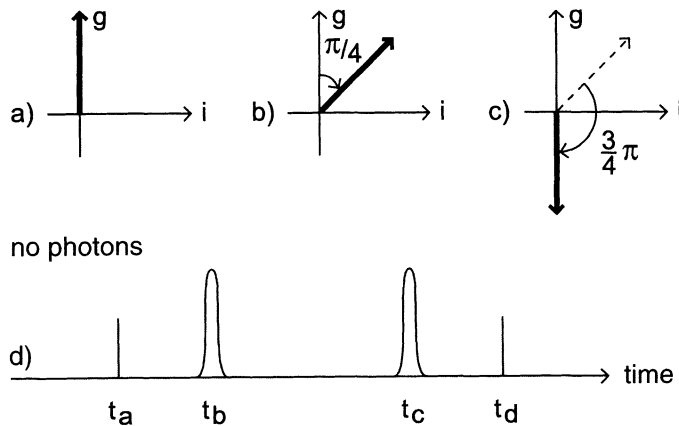
Fig. 22.16 a–d. Explanation of the behavior of the coefficients c of the wavefunction c_g |g, 0\rangle + c_i |i, 0\rangle using a vector diagram. (a) In the initial state, the atom is in the level g . (b) The first pulse rotates the vector (c_g, c_i) by \pi/4 . (c) The second pulse rotates the vector by 3\pi/4 in our picture, so that (apart from a sign) the original state g is again obtained. Finally, the atomic state is measured. Important note: in the interpretation using spins, the rotation angles are twice as large. (d) Temporal sequence of pulses
