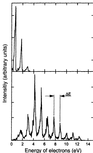
Fig. 15.14. Electronic spectrum of xenon multi-photon ionization. Upper part: At a laser intensity of 2 \cdot 10^{12} W/cm 2 two additional lines show up in addition to the line at E_{\text{kin}} = 0.74 eV. The extra lines are shifted to higher energies by increments given by the energy of the laser photons, \hbar \omega_L . Lower part: If the laser intensity is raised to 10^{13} W/cm 2 more spectral lines appear, which again are shifted relative to each other by increments of \hbar \omega_L . The absolute positions of the spectral lines shift at power output as a consequence of the ponderomotoric energy. (After H. G. Müller et al.)
