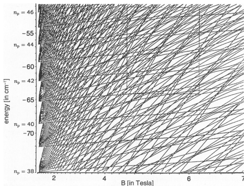
Fig. 14.4. Term scheme of hydrogen atoms in the energy range from -76 \text{ cm}^{-1} to -50 \text{ cm}^{-1} (corresponding to principal quantum numbers 38 \leq n \leq 46 under field-free conditions) as a function of the square of the magnetic field strength. As can be seen, the magnetic multiplets belonging to different principal quantum numbers are intimately intertwined. (After Friedrich and Wintgen, 1989)
