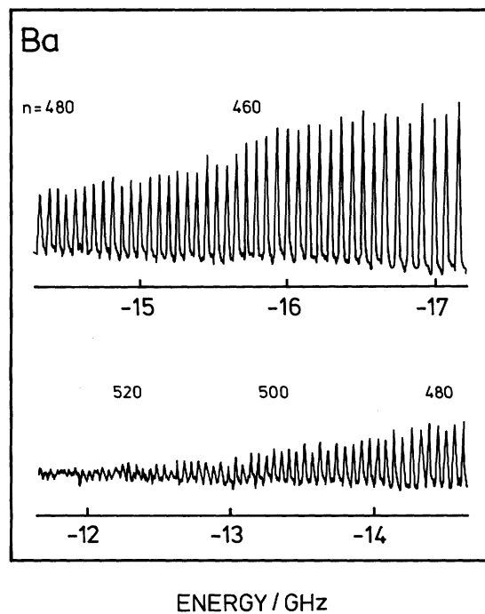
Fig. 8.18. Rydberg excitation states of barium atoms with the principal quantum number n , observed using Doppler-free spectroscopy. The abscissa gives the distance from the series limit in units of GHz. From J. Neukammer et al.: Phys. Rev. Lett. 59, 2947 (1987)
