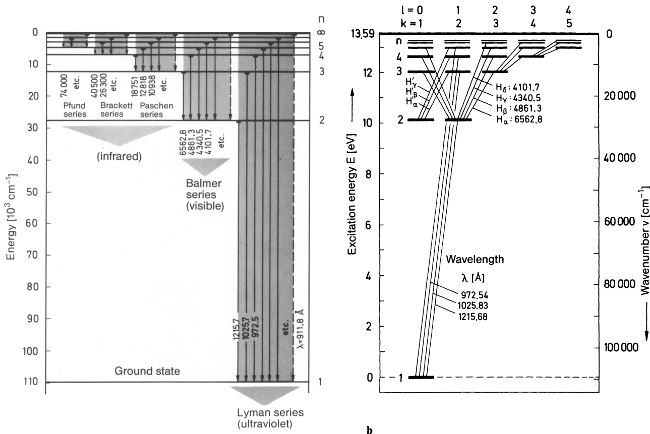
Fig. 8.4. a) Term diagram of the lines of the hydrogen spectrum and series classification. The wavelengths of the transitions are given in Å. The energies can be given as (negative) binding energies, with the zero of energy being the ionisation limit, or they can be given as excitation energies, beginning with the ground state, so that the energy of the term n_\infty is equal to the ionisation energy
