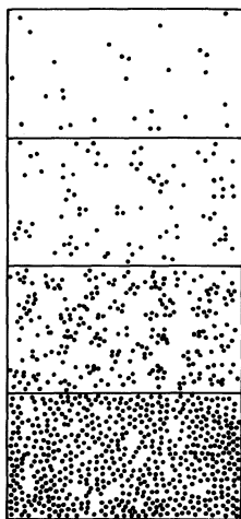
Fig. 2.1. Sedimentation equilibrium: distribution of suspended mastix spheres of 0.6 \mu\text{m} diameter at four different heights in the field of view of a microscope (after Perrin )
