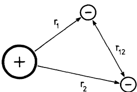
Fig. 19.6. Atom with two electrons
