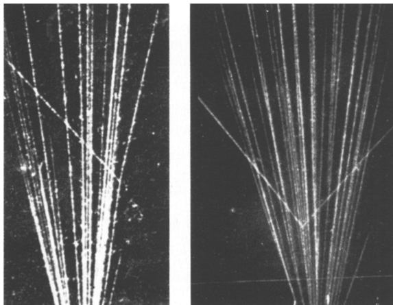
Fig. 4.6. Cloud chamber photographs of alpha particles. Collision processes with the gas in the chamber can be seen; left , the chamber gas is hydrogen, right , it is helium. In hydrogen, the alpha particle is only slightly deflected from a straight-line track, while the hydrogen target nucleus recoils sharply off to the left. In helium, the angle between the tracks of the alpha particle and the recoiling nucleus after the collision is 90^\circ , since the two particles have the same mass. [From K. H. Hellwege: Einführung in die Physik der Atome , Heidelberger Taschenbücher, Vol. 2, 4th ed. (Springer, Berlin, Heidelberg, New York 1974) Fig. 4]
