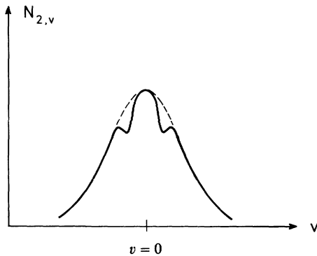
Fig. 22.5. This figure shows the effect of a standing laser wave on the distribution of excited atoms. If we imagine the standing wave to be composed of two travelling waves, each of these components interacts with a group of atoms whose Doppler frequency just coincides with the laser-wave frequency. Therefore, in general, two holes are burned in the distribution. If these two holes overlap, the notch in the distribution is especially deep
