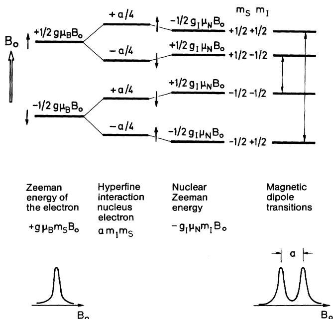
Fig. 20.14. The hyperfine structure of the hydrogen atom in a strong magnetic field B_0 , and the hyperfine structure observable in electron spin resonance (ESR). From left to right, the three contributions to the splitting according to (20.15) are illustrated, along with the magnetic quantum numbers and the allowed (magnetic) dipole transitions. At the lower left, the ESR spectrum of a free electron is shown; at the lower right, that of an electron bound to a proton (H atom). From the splitting in the ESR spectrum, one obtains the hyperfine interaction constant a (in the limiting case of a strong applied field B_0 ). The selection rules for magnetic dipole transitions are \Delta m_S (or \Delta m_J ) = \pm 1 , \Delta m_I = 0 for ESR, and \Delta m_I = \pm 1 , \Delta m_J (or \Delta m_S ) = 0 for nuclear magnetic resonance (NMR)
