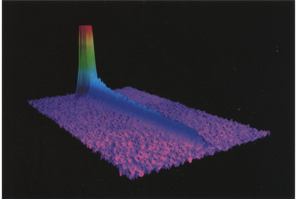
Fig. 23.5. Atom laser: the observed density distribution of a matter-wave beam produced by an atom laser. The coherent atomic beam, which can be seen in the figure as a stretched-out ‘ridge’ extending towards the lower right, is composed of rubidium atoms and originates from a Bose-Einstein condensate. A weak radiofrequency field serves as a continuous and coherent mechanism for extracting the atoms from the condensate; it transfers atoms from the magnetically confined condensate into non-confined states. These atoms escape from the trap and are accelerated by gravity, resulting in a collimated beam of hitherto unattainable brilliance. The region shown in the figure has dimensions of 1.2 \times 2 mm. Because of the high optical density, the image of the condensate distribution (high peak) is saturated. (From Hänsch and coworkers, 1999)
