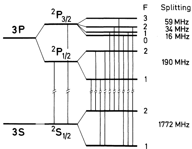
Fig. 20.8. Hyperfine splitting of the lowest terms of the sodium atom with the allowed transitions. The numerical values for the hyperfine splitting are given here in MHz
