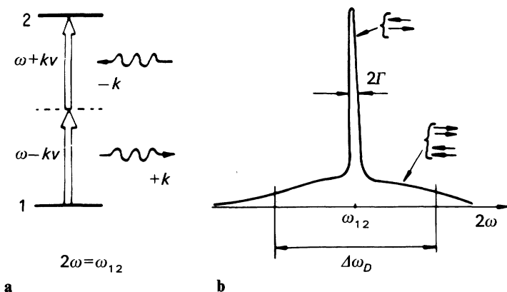
Fig. 22.8. a) Two-photon absorption scheme. We think of the standing laser wave as being broken down again into two waves moving in opposite directions. The part moving to the right interacts with atoms at a Doppler-shifted transition frequency \omega - kv , where k is the wavenumber. The wave moving to the left, however, interacts with the same atom at a Doppler frequency of \omega + kv . When the two waves add, the velocity components cancel out. b) The shape of the resonance line in two-photon absorption. \Delta\omega_D is the Doppler width, and 2\Gamma the total width of the resonance line
