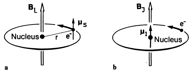
Fig. 20.4. a) Calculation of the spin-orbit interaction: the magnetic moment \mu_s of the electron interacts with the magnetic field of the orbital motion B_L . b) Calculation of the hyperfine interaction: the magnetic moment \mu_I of the nucleus interacts with the magnetic field of the electron shells B_J
