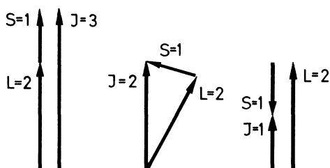
Fig. 17.3. Combination of spin ( S ) and orbital ( L ) angular momenta to form the total ( J ) angular momentum. If L = 2 and S = 1 , J can assume the values 3, 2, or 1. This is a schematic representation. Figure 12.16 explains the method of exact addition of the angular momenta in the vector model
