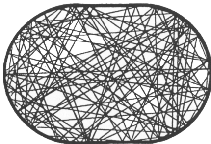
Fig. 14.9. Stadium billiard during which a free moving particle is elastically reflected at the walls is an example of a chaotic system with 2 degrees of freedom. Reflection at the semi-circles causes divergence of neighbouring groups of trajectories. (cf. for instance Ruder et al. , 1994).
