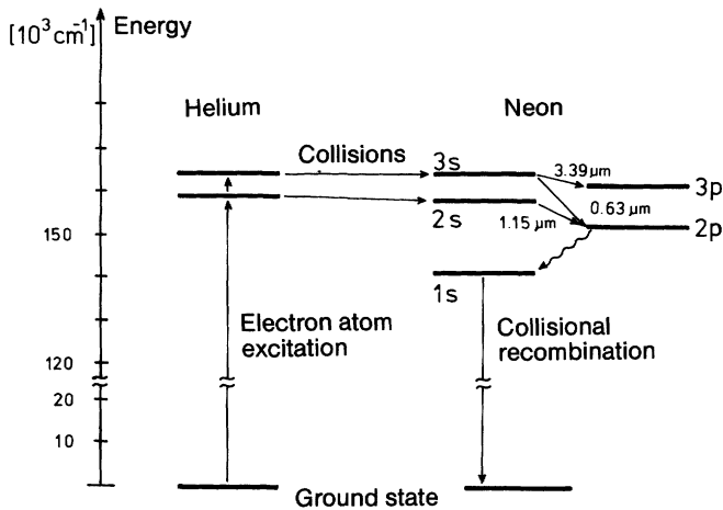
Fig. 21.5. Excitation and recombination processes in the helium-neon laser (schematic). The symbols 1s , 2s , ... used in the neon spectrum on the right are arbitrary technical terms (Paschen symbols) explained in the legend of Fig. 21.6. The helium atoms are excited to the 1S or 3S state by collisions with electrons in a gas-discharge tube. Because the excitation energies correspond to the “ 2s ” and “ 3s ” states of neon, this energy can be transferred from helium to neon by atomic collisions. The electron in the 3s or 2s state in the neon then goes into the 3p or 2p state, and laser light emission may be associated with this process (solid arrows). The electron then drops back to the 1s state by emission of another light quantum. Finally the neon atom loses the remainder of the energy and drops back to the ground state by collisions with other atoms. In reality, the term scheme of neon is much more complicated than shown here (Fig. 21.6). Note that the energy of the ground state was chosen as the zero point of energy here
