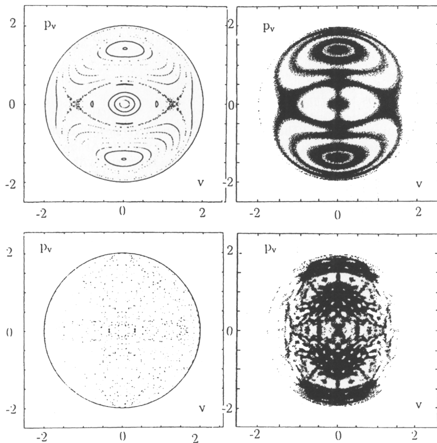
Fig. 14.8. The left side shows the Poincaré cross-sections in semi-parabolic coordinates at scaled energies of \epsilon = -1.0 (upper part) and \epsilon = -0.2 (lower part). The right side shows the cross-section for the quantum mechanical case by means of superimposed Wigner distribution functions for m = 0 eigen states of positive parity with quantum numbers 131 – 135 for \epsilon = -1.0 and quantum numbers 243 – 247 for \epsilon = -0.2 . Note the strong similarity of the classical and the quantum mechanical images for the regular as well as for the chaotic regime. (After Ruder et al., 1994)
