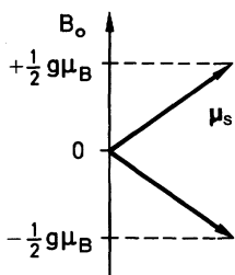
Fig. 13.1. The spin of an electron, and thus its magnetic moment, have two possible orientations in an applied magnetic field. They correspond to two values of the potential energy
