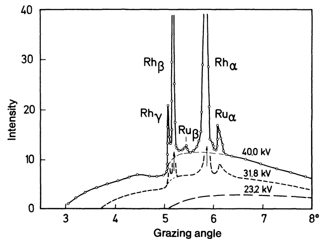
Fig. 18.3. Line spectrum of a Rh anticathode doped with Ru impurity. The lines are superimposed on the bremsstrahlung spectrum. The intensity is plotted against the grazing angle of the crystal spectrometer instead of the wavelength
