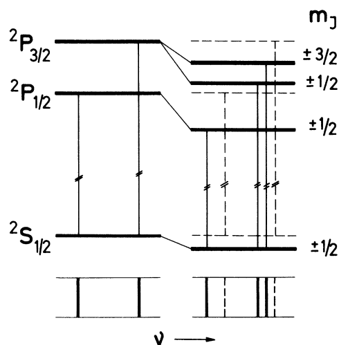
Fig. 15.3. Energy level diagram showing the Stark effect on the sodium doublet 3^2P_{3/2,1/2} - 3^2S_{1/2} and the splitting pattern of the D lines
