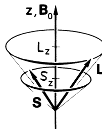
Fig. 13.16. Paschen-Back effect. In the limiting case of a strong magnetic field B_0 , the spin S and orbital L angular momenta align independently with the field B_0 . A total angular momentum J is not defined
