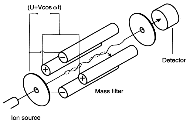
Fig. 3.7. Schematic of a quadrupole mass filter. The ion beam, moving in the +z direction, is deflected by a high-frequency alternating potential. In order for the beam to pass through the filter, a certain relation between e/m , the frequency \omega , and the deflection voltages U and V must be fulfilled. The dashed orbit applies to an ion for which this condition is not met. The electrodes are formed in such a way that they produce an axisymmetric hyperbolic electrostatic field. More on this topic and on the equations describing the movement of ions in such fields can be found in W. Demtröder, Experimentalphysik , Vol. 3, Springer, 1996, Sect. 2.7
