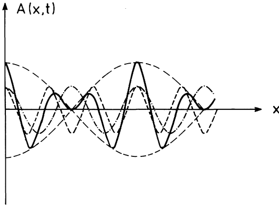
Fig. 7.2. Superposition of two waves of the same amplitude. Fundamental wave 1: (---), fundamental wave 2: (---) same amplitude as 1. Resulting wave A : (—). The envelope \cos(\Delta kx - \Delta \omega t) for constant t is also shown as a dashed curve
