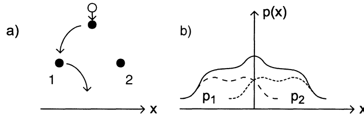
Fig. 23.1. (a) A Galton board with three pins. (b) Probabilities add
