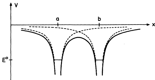
Fig. 24.2. Hydrogen-molecule ion. The potential energy V which acts on the electron due to the attractive forces from nuclei a and b is plotted. The dashed curves show the energy of an electron in the field of nucleus a or nucleus b alone. The full curve is the total potential energy. The abscissa is the position coordinate x . The binding energy of the electron in the field of a single nucleus, E^0 , is also indicated
