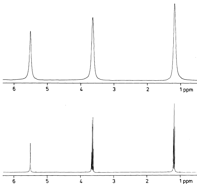
Fig. 20.20. Nuclear magnetic resonance (NMR) of ethyl alcohol, C_2H_5OH . The signal intensity at the receiver is plotted against the transition frequency. The latter is measured in ppm (parts per million) relative to the frequency of a suitable standard. In the upper portion of the figure, one sees three lines having the intensity (area) ratio 1 : 2 : 3. They are due to proton spins in the -OH , the -CH_2 , and the -CH_3 groups, respectively, having 1, 2, and 3 protons. The resonance frequencies of these protons differ by a few ppm due to the differing chemical bonding in the three groups. In the lower portion, the same spectrum, but with higher experimental resolution, is shown. The -CH_2 signal is now split into a quartet of lines by the interaction with the -CH_3 protons, while the signal from the latter is split into a triplet by the indirect nuclear spin interaction with the -CH_2 protons. The protons of the -OH groups are rapidly exchanged between different molecules, which averages out the indirect spin interactions and leaves a single resonance line
