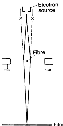
Fig. 6.9. Electron interference with an electrostatic double prism according to Möllenstedt and Düker . There is a voltage between the fibre and the counterelectrodes. The electrons are deflected by the resulting inhomogeneous field as shown. From Gerthsen, Kneser, Vogel: Physik , 13th ed. (Springer, Berlin, Heidelberg, New York 1977) Fig. 10.68
