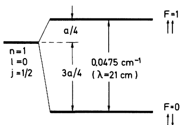
Fig. 20.7. Hyperfine structure of the hydrogen ground state. The spins of electrons and protons can be parallel or anti-parallel to each other. See also Sect. 12.1
