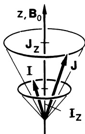
Fig. 20.12. Hyperfine structure in a magnetic field. Vector diagram of the Paschen-Back effect. A total angular momentum F is no longer defined
