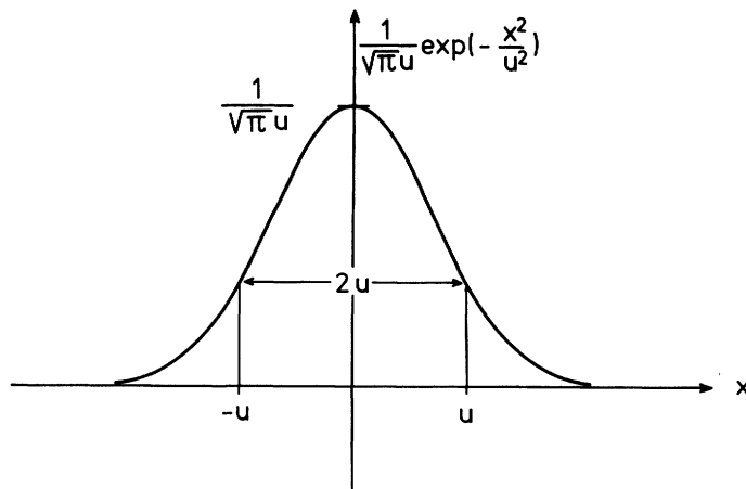
Fig. A.1. The function (1/\sqrt{\pi u}) \exp(-x^2/u^2) plotted against the variable x . If we let the parameter u become smaller, the value of the function at x = 0 gets larger and larger and the decrease to both sides gets steeper, until the function has finally pulled itself together into a \delta function
