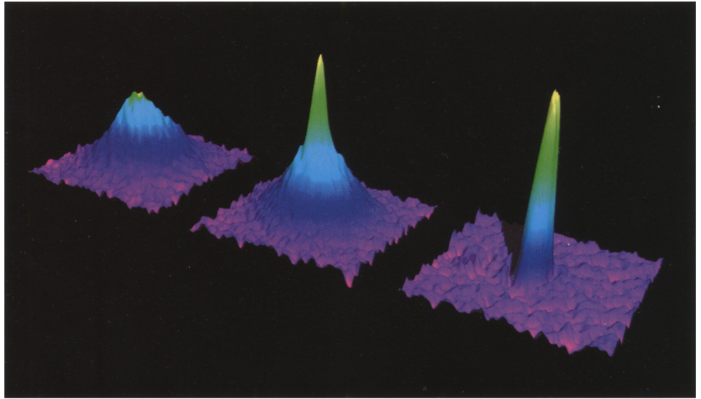
Fig. 23.4. Bose-Einstein condensation: the measured density distribution of the cold atoms near the phase transition to a Bose-Einstein condensate. The image on the left was taken at a temperature slightly above the critical temperature T_C , the middle one just at T_C , and the right image far below T_C . Each image represents an area of 600 \times 600 \mu\text{m} . These images of the density distribution were taken after 17 ms of ballistic expansion of the atomic cloud following switching off of the magnetic trap (from Th. Hänsch et al. 1999)
