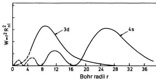
Fig. 11.8. Radial probability densities for a 4s and a 3d electron in the H atom. The 4s electron is, on the average, farther from the nucleus, but the probability of finding it near the nucleus is greater than the probability of finding the 3d electron there
