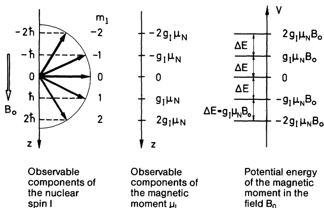
Fig. 20.2. The nuclear spin I (here for the case I = 2 ) has discrete orientations relative to a special direction, here an externally applied magnetic field B_0 (left). Correspondingly, the measurable component of the magnetic moment (middle) and the potential energy (right) have discrete values
