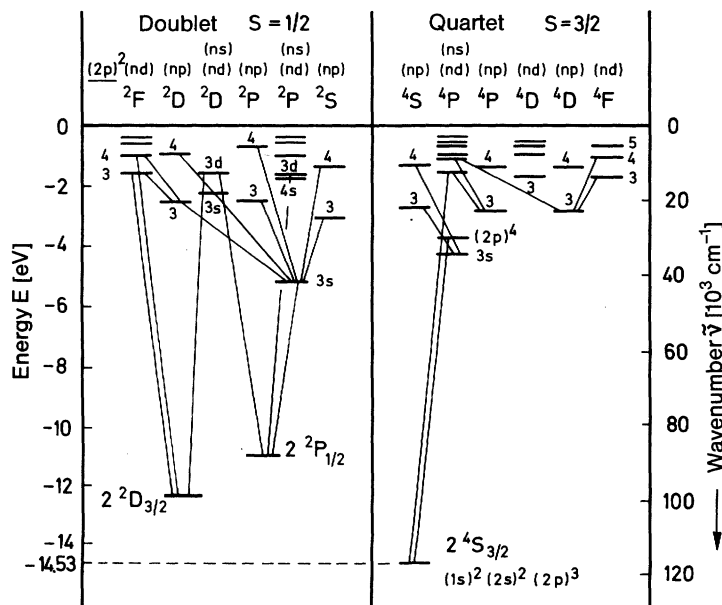
Fig. 17.4. Term diagram for the nitrogen atom (only simple terms, no J splitting). Nitrogen as a doublet and a quartet system. The electronic configuration of the valence electrons is given at the top
