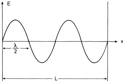
Fig. 21.2. Standing wave between the mirrors of the laser
