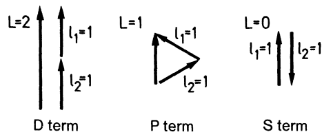
Fig. 17.2. Coupling of the orbital angular momenta of two electrons l_1 and l_2 to the total angular momentum L . Coupling to D , P and S , corresponding to L = 2, 1 , and 0 . The picture is schematic. Exact addition of the angular momenta is accomplished as shown in Fig. 12.16
