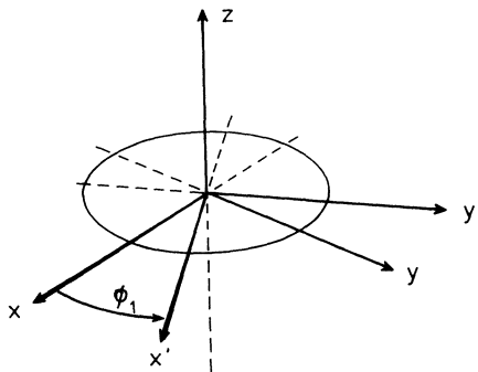
Fig. 16.3. Rotation of the coordinate system around the z axis by an angle \phi_1
