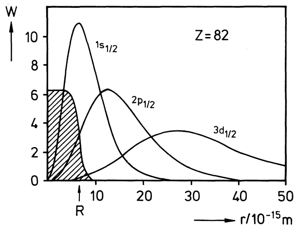
Fig. 8.8. The probability W of finding a muon at a distance r from the center of the nucleus of a muonic atom, in arbitrary units, for various shells; also showing the nuclear charge distribution ( shaded area ). The plot is for the lead nucleus, with Z = 82 and nuclear radius R = 6.687 \cdot 10^{-15} \text{ m (fm)} . The symbols used to indicate the shells will be explained later. (After E. Boric and G.A. Rinker: Rev. Mod. Phys. 54 , 68 (1982))
