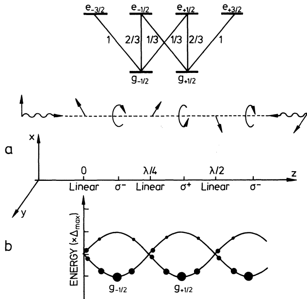
Fig. 22.12. Line shifts in a polarization gradient. (a) Counter-propagating laser beams with mutually orthogonal linear polarizations create a total field which alternates from linear to circular polarization along each eighth of a wavelength. The upper part of the figure shows the energy levels of the atom considered. The numbers on the lines connecting the different ground ( g ) and excited ( e ) sublevels indicate the relative transition probabilities. (b) The energies, shifted as described in the text, and the populations of the two ground state sublevels of this atom. The energies and populations change with the polarization of the light and thus with the position of the atom along the beam. The size of the population is symbolized by the size of the circles. (After Claude N. Cohen-Tannoudji and William D. Phillips: Physics Today , pp. 33–40 (1990))
