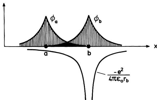
Fig. 24.5. Intuitive explanation of the integral (24.9). The three functions \phi_a , \phi_b , and -e^2/(4\pi\epsilon_0 r_b) which occur in the integral are plotted. Since the product of these three functions occurs, nonvanishing contributions are only possible when the wavefunctions \phi_a and \phi_b overlap, as is indicated by the heavily shaded area. The integral is obtained by multiplying the functional values of \phi_a , \phi_b , and -e^2/(4\pi\epsilon_0 r_b) at each point in space and adding up over the whole volume
