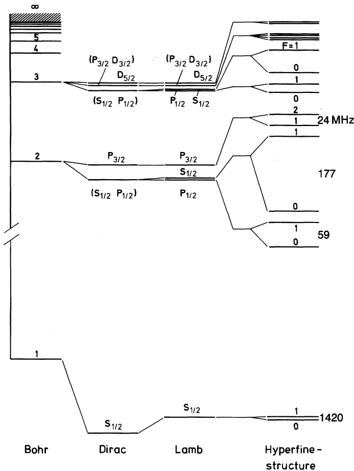
Fig. 20.6. Term diagram of the H atom including the hyperfine splitting. All fine structure terms (see Fig. 12.20) are doubly split by the interaction with the proton. The magnitude of the splitting is not drawn to scale here. In particular, the scale was enlarged on going from the Bohr energy levels to the fine structure and again in going to the hyperfine structure, in order to show the energy differences which become smaller and smaller from left to right. The scale increases from below to above in the case of the hyperfine splitting; the latter is largest in the ground state, n = 1 . The numerical values of the hyperfine splittings are given in MHz
