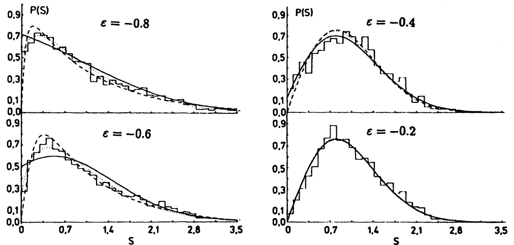
Fig. 14.10. Histograms P(S) of level distances of the hydrogen atom in magnetic fields at different values of the scaled energy (after Wintgen and Friedrich, 1987). The unbroken curves result from fittings by means of various formulas derived in the literature for the purpose of interpolating Poissonian and Wigner distributions. (After Ruder et al. , 1994)
