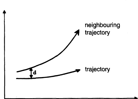
Fig. 14.6. The figure shows a section of phase space in two dimensions. If the Lyapounov exponent is positive, the distance of two neighbouring trajectories will grow exponentially.
