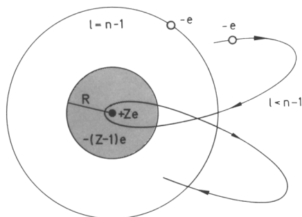
Fig. 11.4. Variation in screening for electrons with different radial probability densities. In the Sommerfeld model it is intuitively clear that electrons with “diving orbits” approach the nucleus closely and are affected at least partially by the unscreened nuclear potential. It has to be remembered, however, that in the modern quantum theory, the electrons are described as charge clouds rather than as orbiting particles
