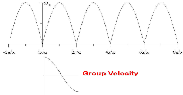
Dispersion relation in extended zone
