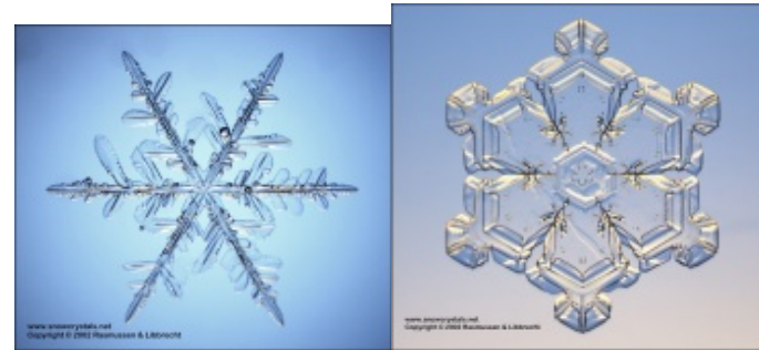
Snow crystals.
