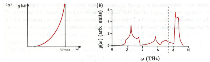
Figure The density of normal modes in a three-dimensional crystal. (a) The Debye model, (b) The density of states for Ge, as calculated with the adiabatic bond charge model (Weber 1977).
