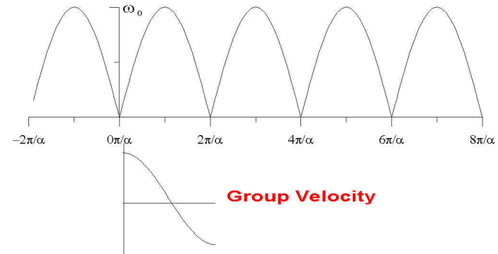
Dispersion relation in extended zone
