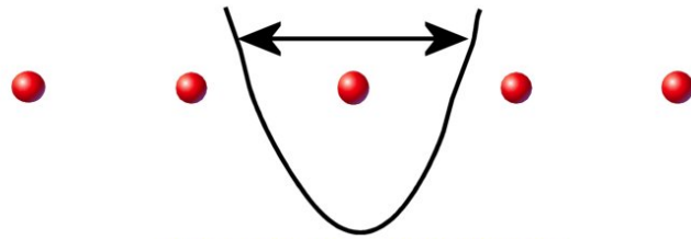
All atoms except one fixed - Einstein model
