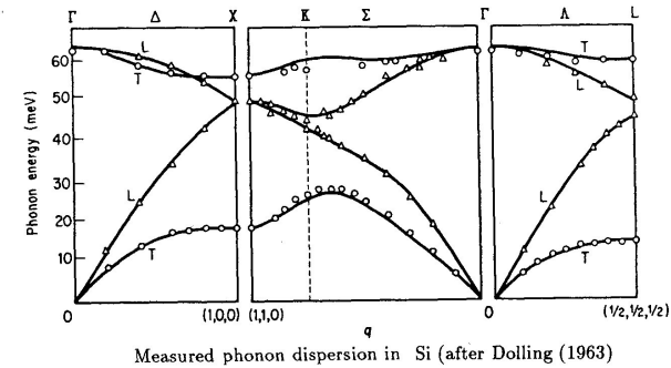
Measured phonon dispersion in Si (after Dolling (1963))
